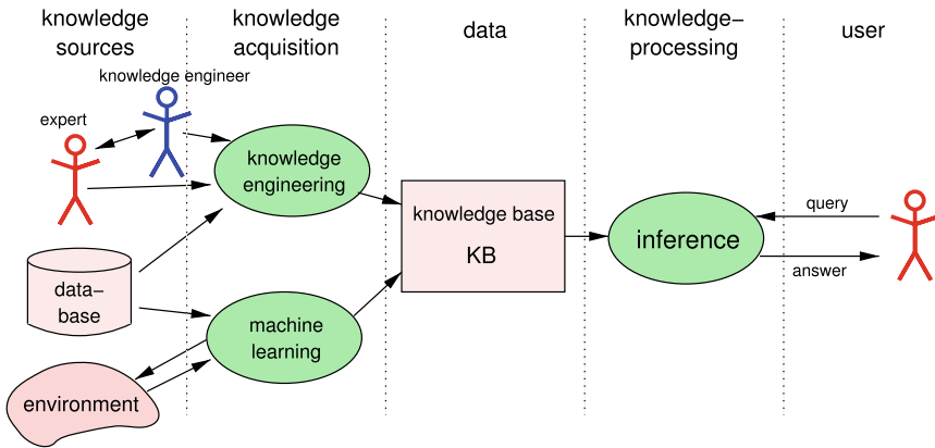
Fig. 1.7 Structure of a classic knowledge-processing system
