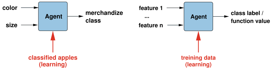
Fig. 8.4 Functional structure of a learning agent for apple sorting ( left ) and in general ( right )
